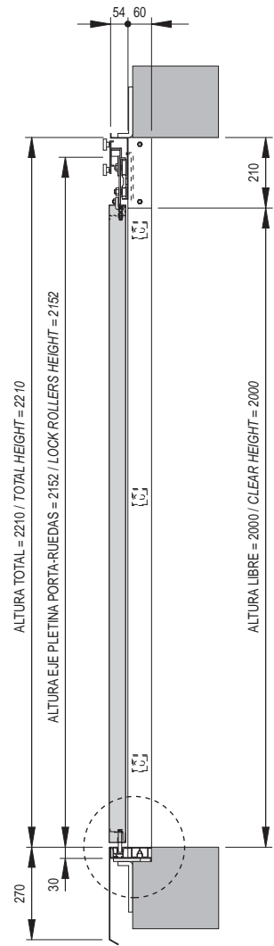
DETALLE PISADERA FLUSH SILL AND TRACK DETAIL
